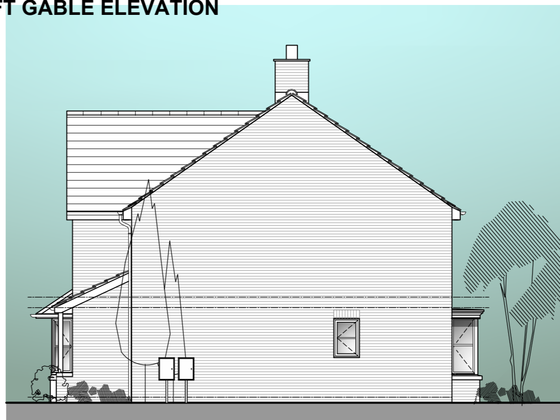
RIGHT GABLE ELEVATION
