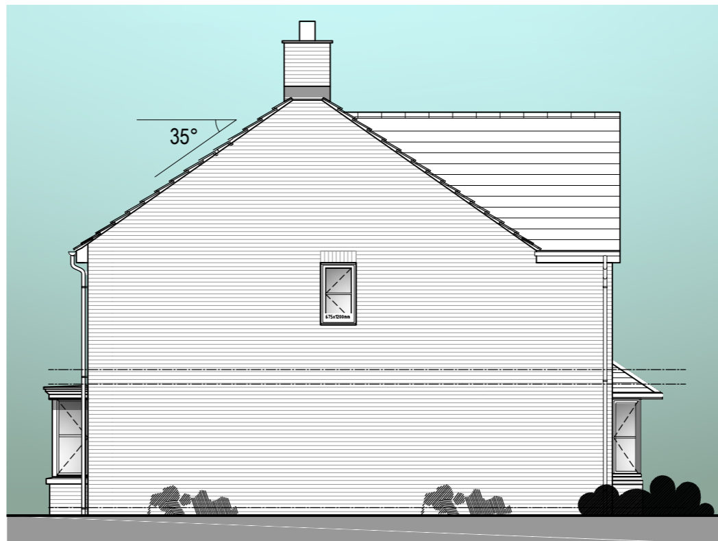
LEFT GABLE ELEVATION
